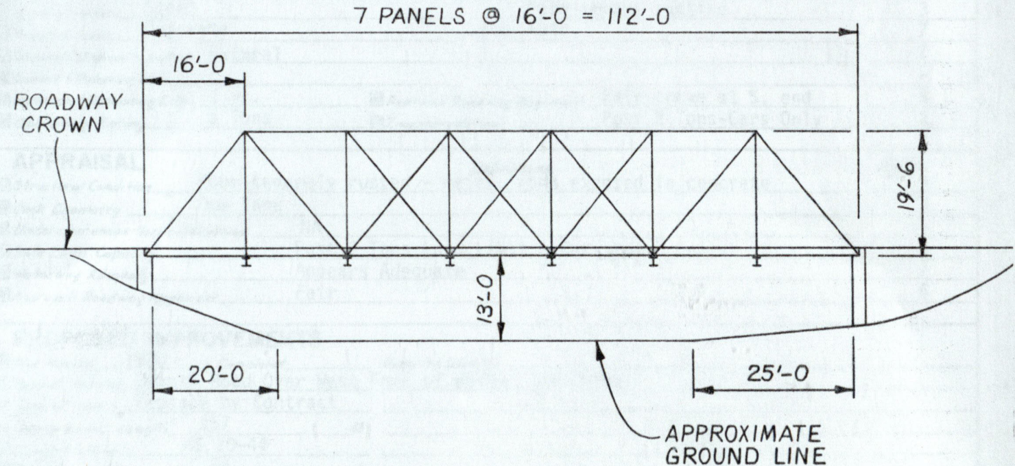
LOOKING SOUTHWEST BRIDGE NO. 182 WARREN TRUSS
